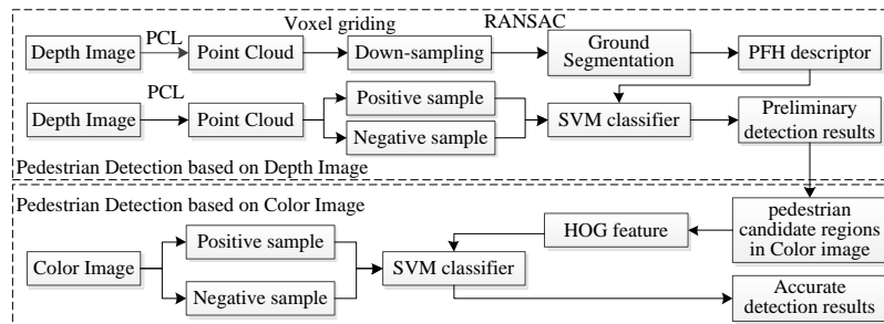
Fig. 1. Algorithm flow
