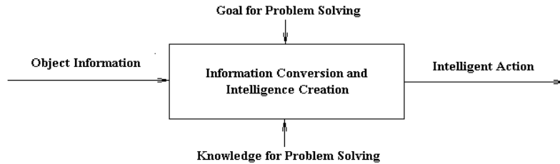
Fig. 3. Another Expression for the Formula (4.1)
