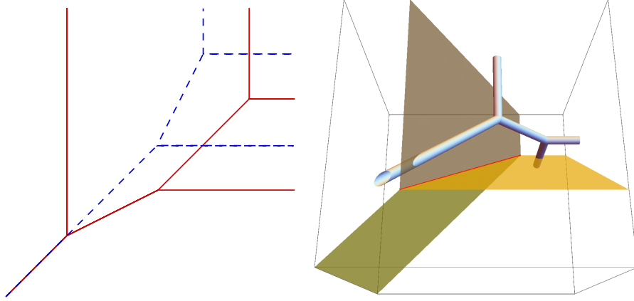
FIGURE 1. Left: Tropicalizations of the equations for two circles in Example 1 always intersect non-transversely, even when the coefficients a_1, \dots, a_8 are generic Puiseux series.
