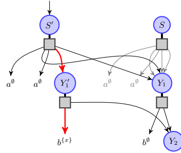
Fig. 9: G' on \Sigma^{\mathbb{V}} with pat(G') = pat(G) * [x/5] .
