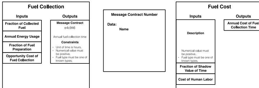
Fig. 2. Illustration of model input/output and matching message contract.
