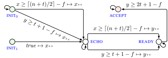
Figure 1. A threshold automaton for Byzantine agreement [4]
