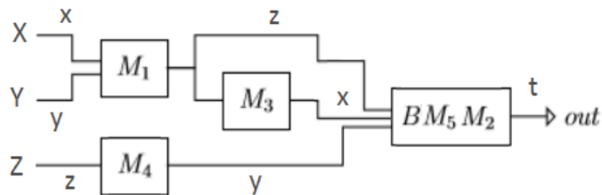
Fig.7. Reduction step 1
