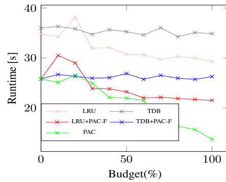
Fig. 6: Runtime on u-ssb-80k
