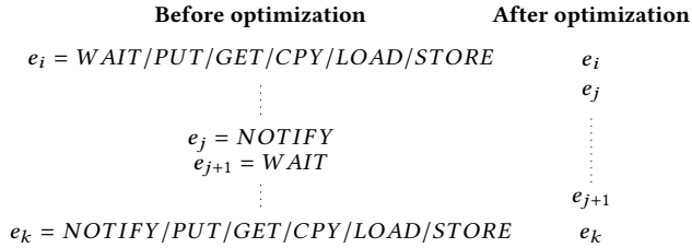
Figure 3: Code transformation for barriers optimization.
