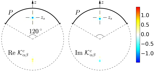
Fig. 2. Meridional slice through the sound-speed kernel \mathcal{K}_{\alpha\beta}^c(\mathbf{x}, r_s) computed in Model S at a single frequency of 3 mHz, in units of 10^{-34} \text{ kg m}^{-3} \text{ s}^{-3} . Both the real (left panel) and imaginary (right panel) parts of the kernel are shown. The scatterer at z_s = 0.7 R_\odot is indicated by the crosses. The observation pupil P is a polar cap of full angular size 120^\circ . Notice the ghost values at the antipode result from the reflection of waves at the surface due to the rapid drop of the density.
