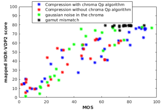
Fig. 2: HDR-VDP2 scores in function of the MOS.
