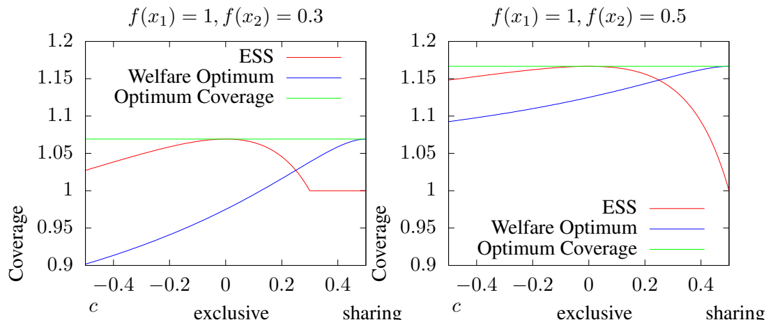
Figure 1: Coverage as a function of the extent of competition (parametrized by c ) for the case where two players complete over two sites x_1 and x_2 . On the left (respectively, right) we consider the case where f(x_1) = 1 and f(x_2) = 0.3 (respectively, f(x_2) = 0.5 ). The X -axis represents a range of congestion functions C_c , defined as C_c(1) = 1 and C_c(2) = c , where c \in [-0.5, 0.5] . The case c = 0 corresponds to the exclusive function and the case c = 0.5 corresponds to the sharing function. The Y -axis represents the coverage. The red line corresponds to the coverage of the ESS, the green corresponds to the optimum coverage, taken over all symmetric strategies, and the blue corresponds to the coverage of the symmetric strategy that maximizes the individual payoffs.
