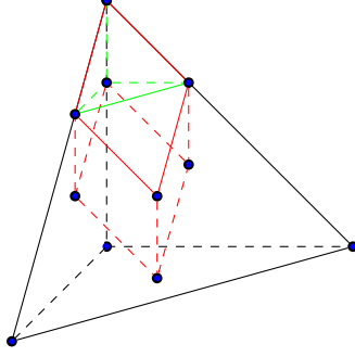
Figure 2: Subdivision of the unit simplex used in the proof of Theorem A.2. The unit simplex is shown for d = 3 , along with its sub-simplex K_\dagger (edges shown in green) and sub-parallelepiped Q_\dagger (edges shown in red).
