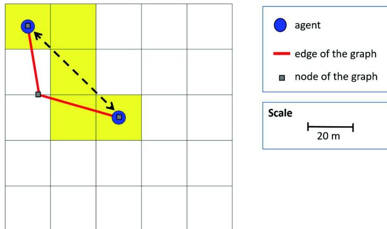
Fig. 4 Computation of distances between two agents (blue circle) according to different GAMA topologies : distance with the continuous topology (Euclidean): 56.6 m; distance with the grid topology (yellow cells): 4 cells, distance with the graph topology (red lines representing roads): 66.8 m
