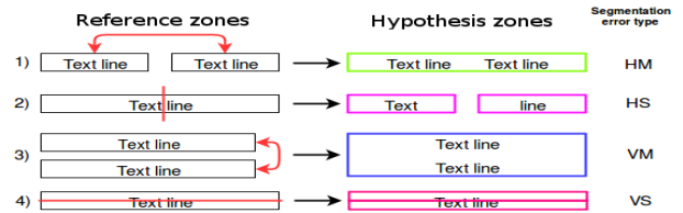
Figure 1: Segmentation errors at line level. HM is horizontal merge. HS is horizontal split. VM is vertical merge. VS is vertical split.
