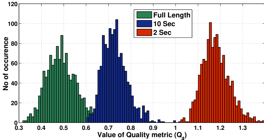
Figure 4: Distribution of quality measure Q_4 for 2 sec, 10 sec, and full segment, estimated from NIST 2008 short2 enrollment corpus.
