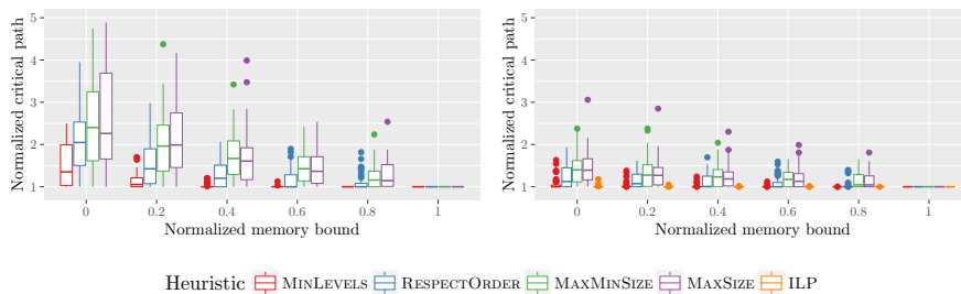
Figure 4: Critical path length obtained by each method for the DAGGEN dataset (left:sparse, right:dense).
