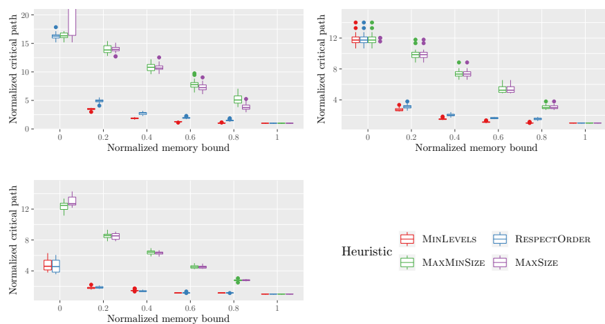
Figure 5: Critical path length obtained by each method for the LIGO (top left), GENOME (top right) and MONTAGE (bottom) datasets. Critical path and memory normalized as in Figure 4.
