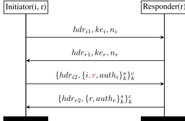
Fig. 5. The IKEv2-Sig-IDr protocol. We make IDr ( r in the figure above) payload mandatory in the IKE_AUTH request and modify its processing by Responder.
