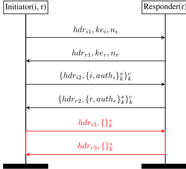
Fig. 6. The IKEv2-Sig-conf protocol. We add the key confirmation exchange. Connections are installed only after this exchange.
