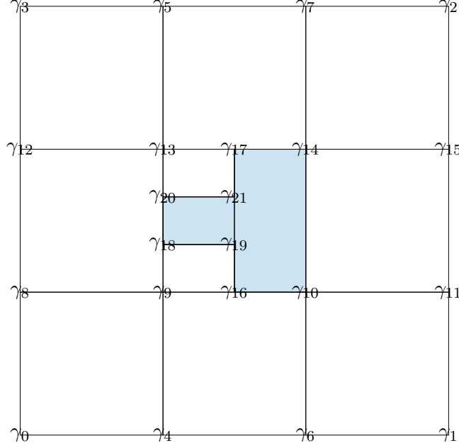
Figure 8: A non-uniform degree C^2 spline space consisting of cubic and quartic polynomial pieces is built on the above mesh. Example 8.3 shows that the dimension of the spline space coincides with the upper bound implied by Theorem 7.2.
