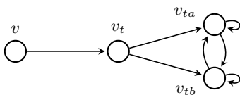
Fig. 5. An abstract graph for the RPN in Figure 1
