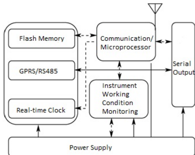
Fig. 4. Composition of the Data Forwarding Unit
