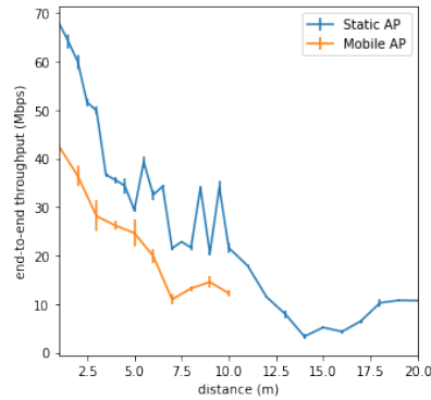
Fig. 5: Average E2E throughput with respect to the distance.
