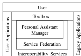
Fig. 1. ARISA Reference Model
