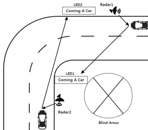
Fig. 1. Simulation system
