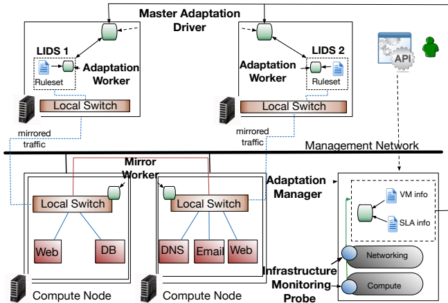
Fig. 1. SAIDS architecture
