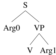
Figure 2: Organisation of the main constituents in FRMG
