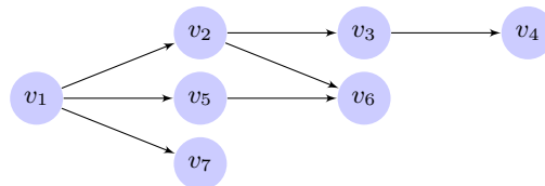
Figure 1: DAG example.
