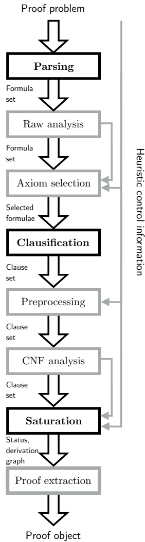
Fig. 1. Logical pipeline
