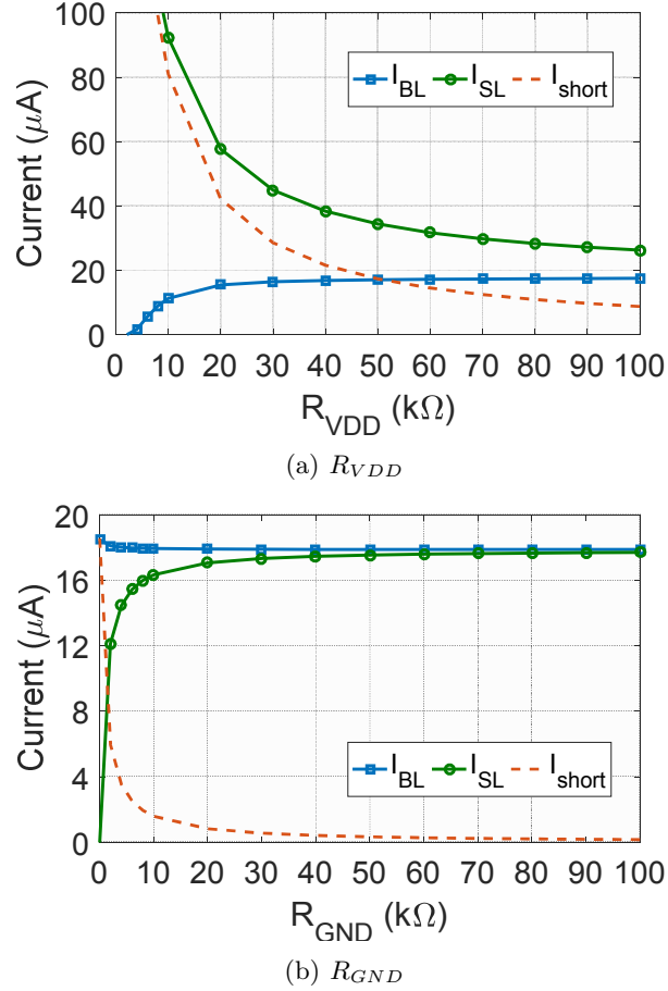
Fig. 13. Behavior of BL and SL currents as function of the short defect resistance.
