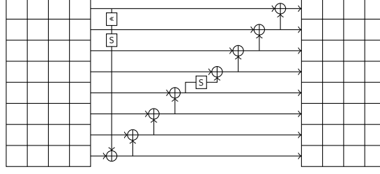
Figure 5: AES-256 key schedule [Jea16]
