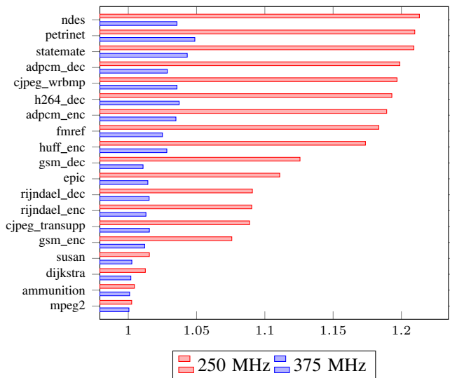
Fig. 2: Performance degradation when memory speed is set at different frequencies
