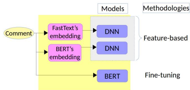
Fig. 1. Proposed methodology
