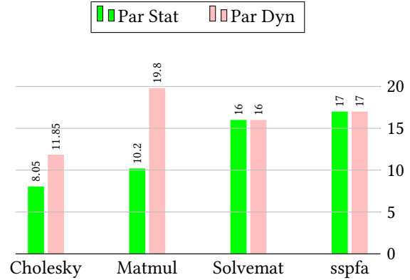
(a) Execution time for config1 machine (seconds)
