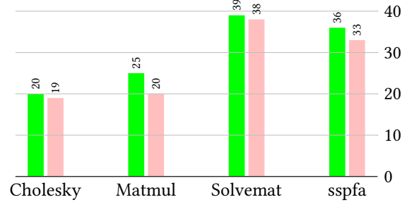
(b) Execution time for config2 machine (seconds)
