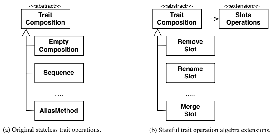
Figure 7: Extensible trait composition algebra: the original stateless trait operations are implemented in an extensible way (a) and are extended to support stateful trait operations (b).
