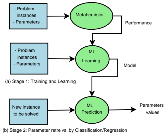
867 Fig. 9. ML and parameter tuning: training, learning and prediction. 868
