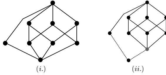
Fig. 2. Illustration of the proof of Corollary ??. For the lattice in (i), each filter is distributive and so L \setminus \perp is a distributive \vee -semilattice. However, the second condition is not satisfied. One possibility is to keep \perp but the whole lattice should be then distributive (which is not the case). The other possibility is to add a new infimum distinct from \perp . In this case, the poset of \vee -irreducible elements is not invariant from (i) to (ii).
