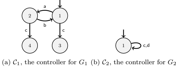
Fig. 6. Modular controllers produced using Algorithm 3 to enforce the opacity of \mathcal{S}_1 and \mathcal{S}_1 w.r.t. G_1||G_2 and \Sigma_a
