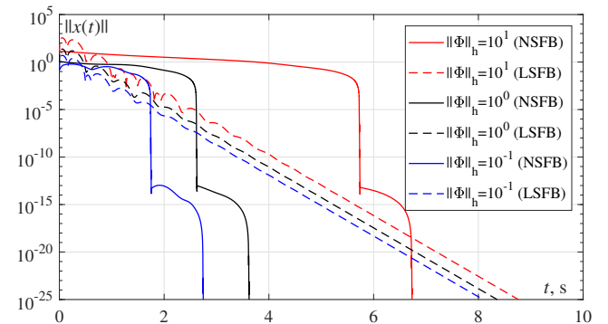
Fig. 1. Comparison of nonlinear (NSFB) and linear state feedback (LSFB) for different initial conditions
