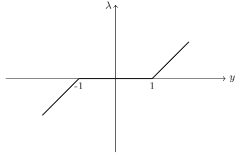
Fig. 7 Deadzone characteristic
