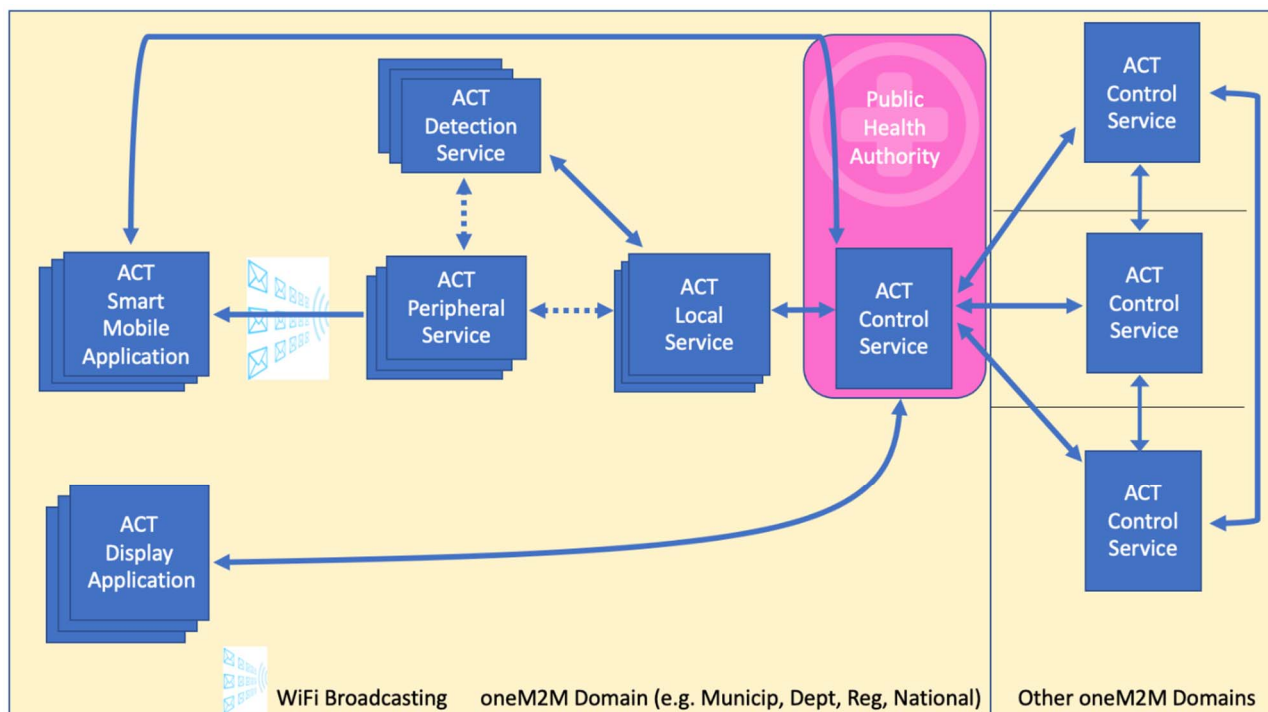
Figure 5.1-1: ACT Architecture
