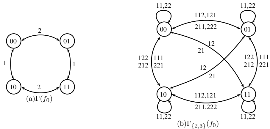
Figure 2. Iterating f_0 : (x_1, x_2) \mapsto (\overline{x_1}, \overline{x_2})
