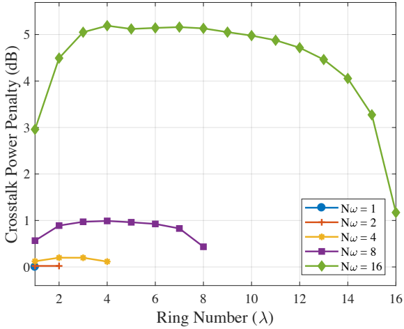
Fig. 2. Crosstalk power penalty repartition for each signal of a N_w wavelengths receiver.
