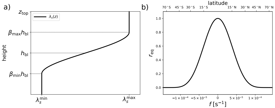
Figure 1. a) Typical profile of the nudging coefficient \lambda_s(z) with respect to the parameters \lambda_s^{\max}, \lambda_s^{\min}, \beta_{\min}, \beta_{\max}, h_{bl} . b) Equatorial restoring function r_{eq} with respect to the Coriolis frequency f .
