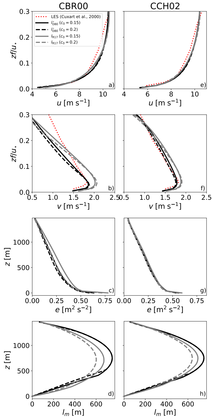
Figure 4. Results obtained for the neutral boundary-layer case of Andren et al. (1994) with the CBR00 model constants (left panels a to d) and CCH02 model constants (right panels e to h) for different parameter values for c_0 and different mixing length formulations ( l_{D80}^* for black lines or l_{R17} for grey lines). Results are shown for u (panels a & e), v (panels b & f), e (panels c & g), and l_m (panels d & h). In the top four panels results are compared with LES simulations from Cuxart et al. (2000) (their Fig. 16). As in Andren et al. (1994), simulations were run over a period of 10/f and results are averaged over the last 3/f period.
