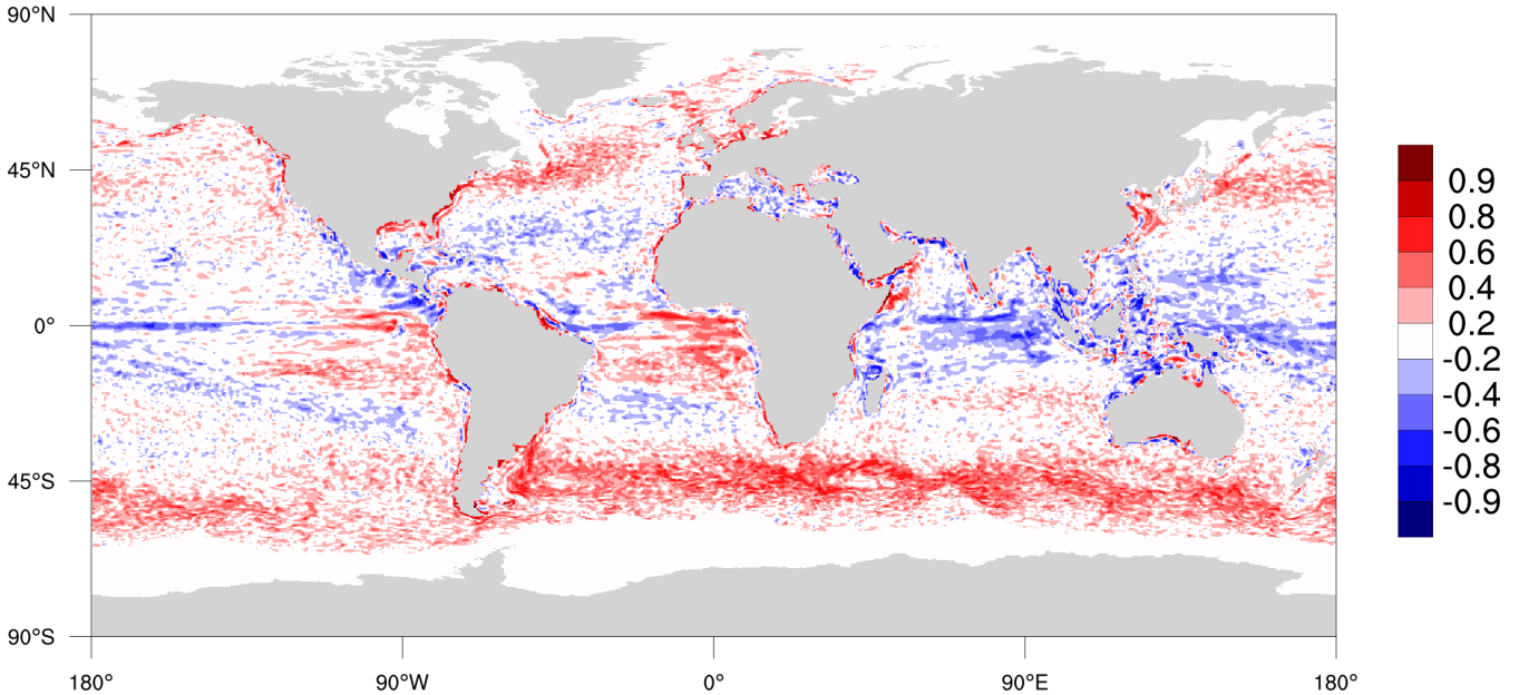
Figure 10. Global map of temporal correlation of high-pass filtered wind speed at the first vertical level of the ABL1d model with SST from NEMO. Both NEMO and ABL1d are configured at 0.25^\circ resolution.
