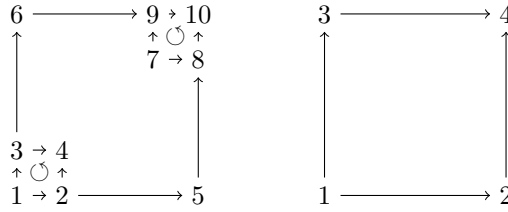
Figure 5: Category of components of SF and HS
