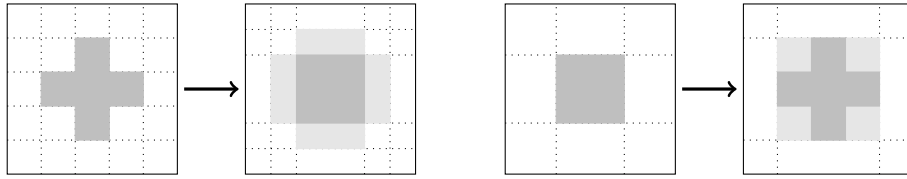
Figure 2: dmap from SF to HS (left) and from HS to SF (right)
