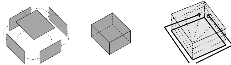
Figure 3: Fahrenheit's matchbox M and two non-dihomotopic dipaths
