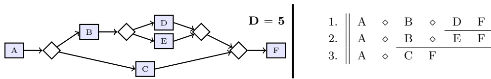
■ Figure 7 A C-DAG instance with two conditional constructs. Each vertex has WCET=1, and all are assigned to the same processor. Its “certificate” of feasibility is shown on the right: it comprises three schedules, all of which are identical until the first conditional construct is executed (depicted as a \diamond ). The top two schedules, which correspond to the upper branch being taken, are further identical until the second conditional construct is executed.
