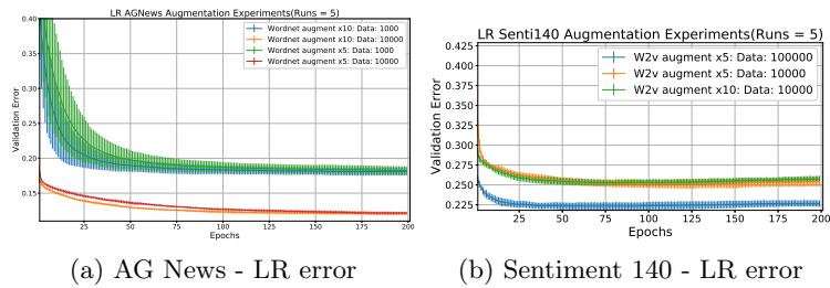
Fig. 5. Effects of different sizes of augmentation given different input data on error. (a) WordNet-based augmentation slightly reduces the error with more number of augmentations. (b) Word2Vec increase the error by introducing more noise.
