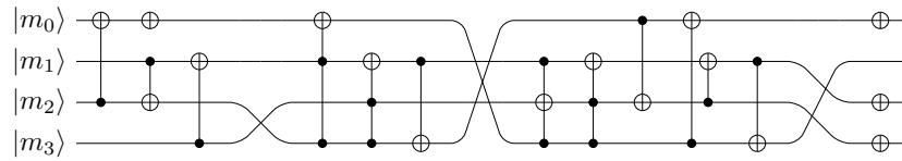
Circuit 7 The SPONGENT S-box.
