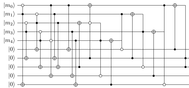
Circuit 8 KECCAK's \chi function.
