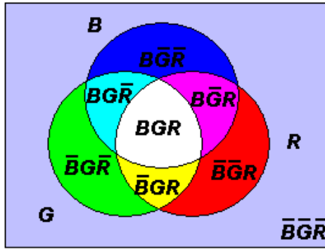
Fig. 4. Venn's diagram showing the logic operations of the opponent-process.
