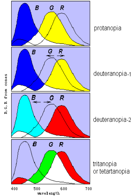
Fig. 7. Different kinds of color blindness illustrated by incomplete separations of three sensitive curves.
