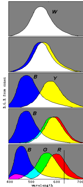
Fig. 6. The Evolution of color vision illustrated by splitting sensitivity curves.
