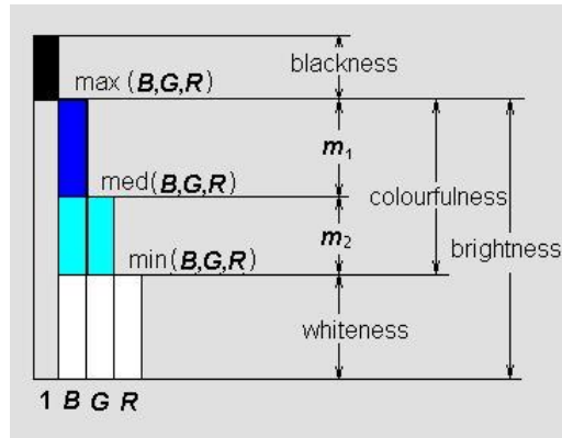
Fig. 3. Relationship between B, G, R and brightness, colorfulness, whiteness, and blackness.
