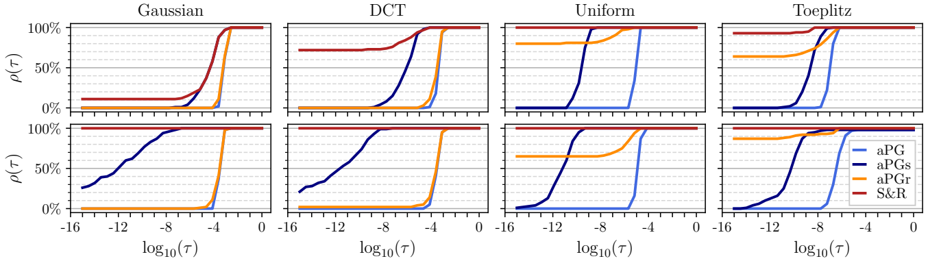
Fig. 1. Dolan-Moré performance profiles for (\lambda, \varepsilon) = (0.2, 0.5)\lambda_{\max} (top) and (\lambda, \varepsilon) = (0.5, 0.2)\lambda_{\max} (bottom).
