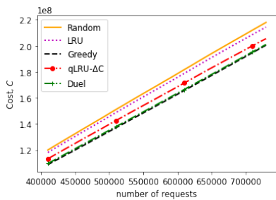
Fig. 7. Performance of different policies under Amazon trace.
